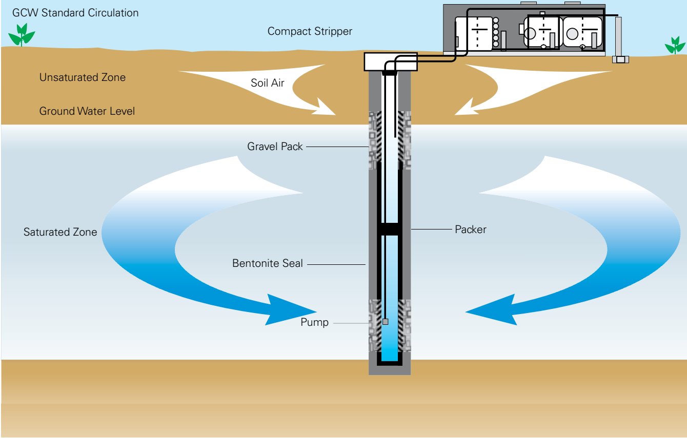
Figure 2.2: Infiltration well or French well
