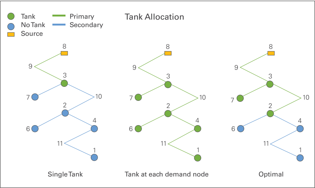
Figure 4C.4: Alternate tank/ESR configurations for a sample network
