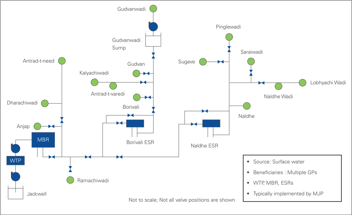
Figure 4A.2: Schematic layout of Sugave multi village scheme
