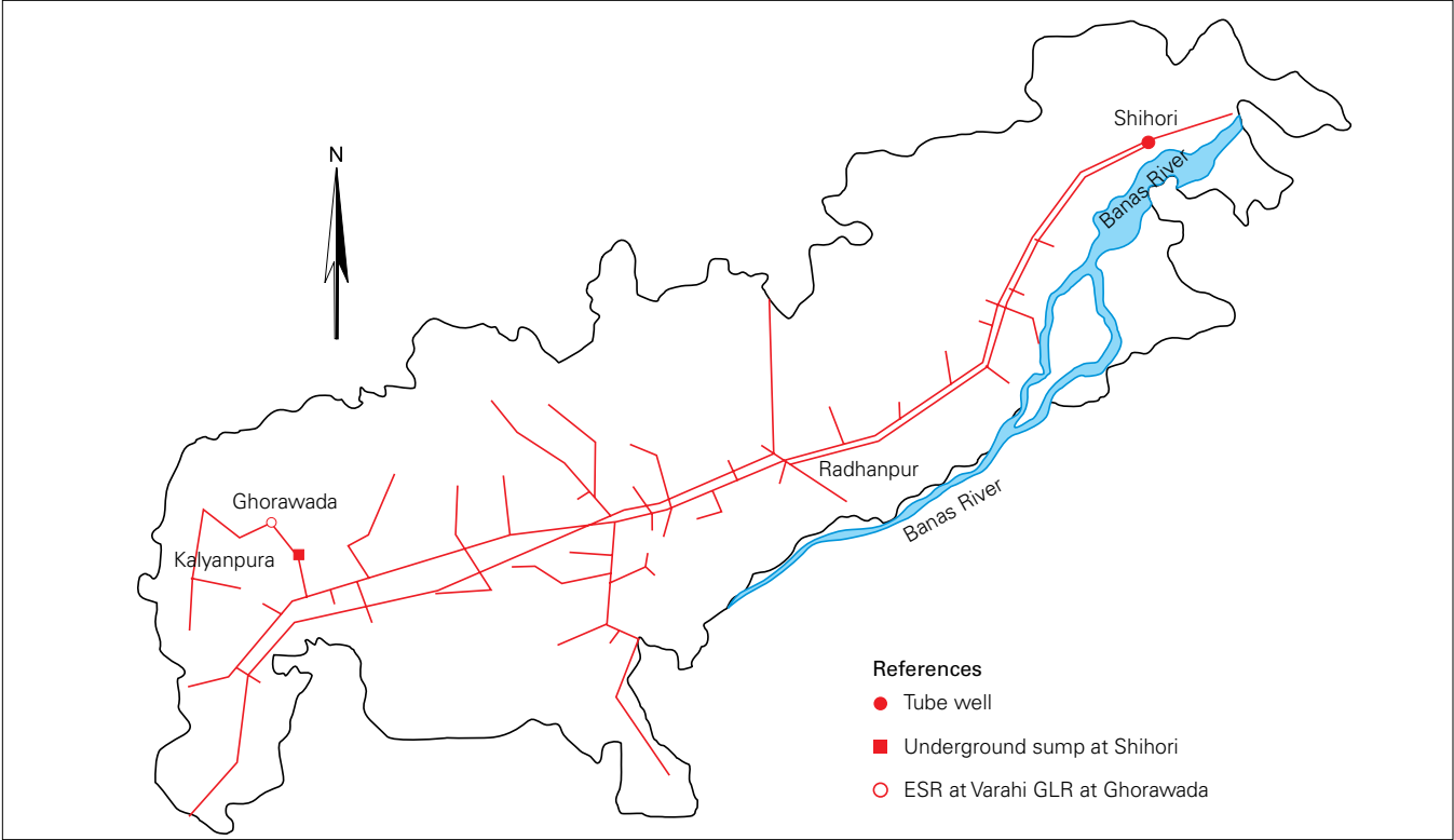
Figure 2.1: Schematic lay out of distribution network of Santalpur regional water supply scheme
