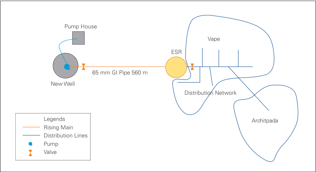
Figure 3C.4: Schematic layout of the scheme
