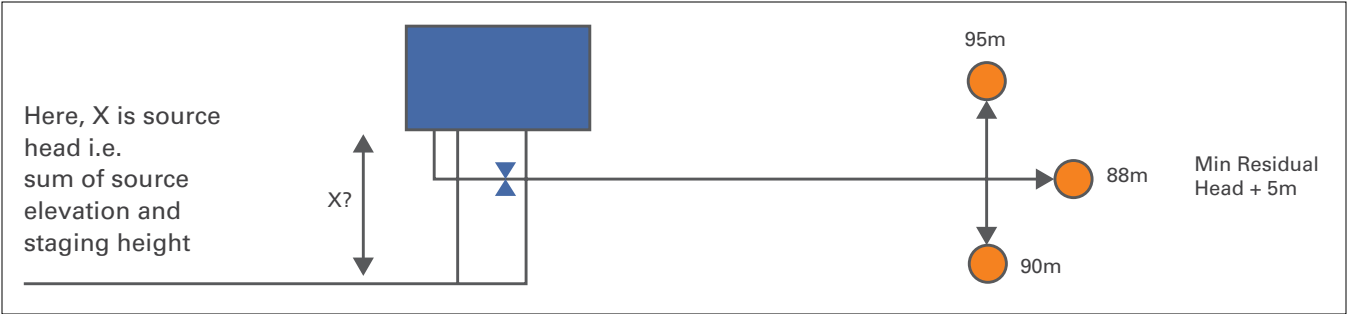
Figure 4A.4: Staging height as per minimum residual head
