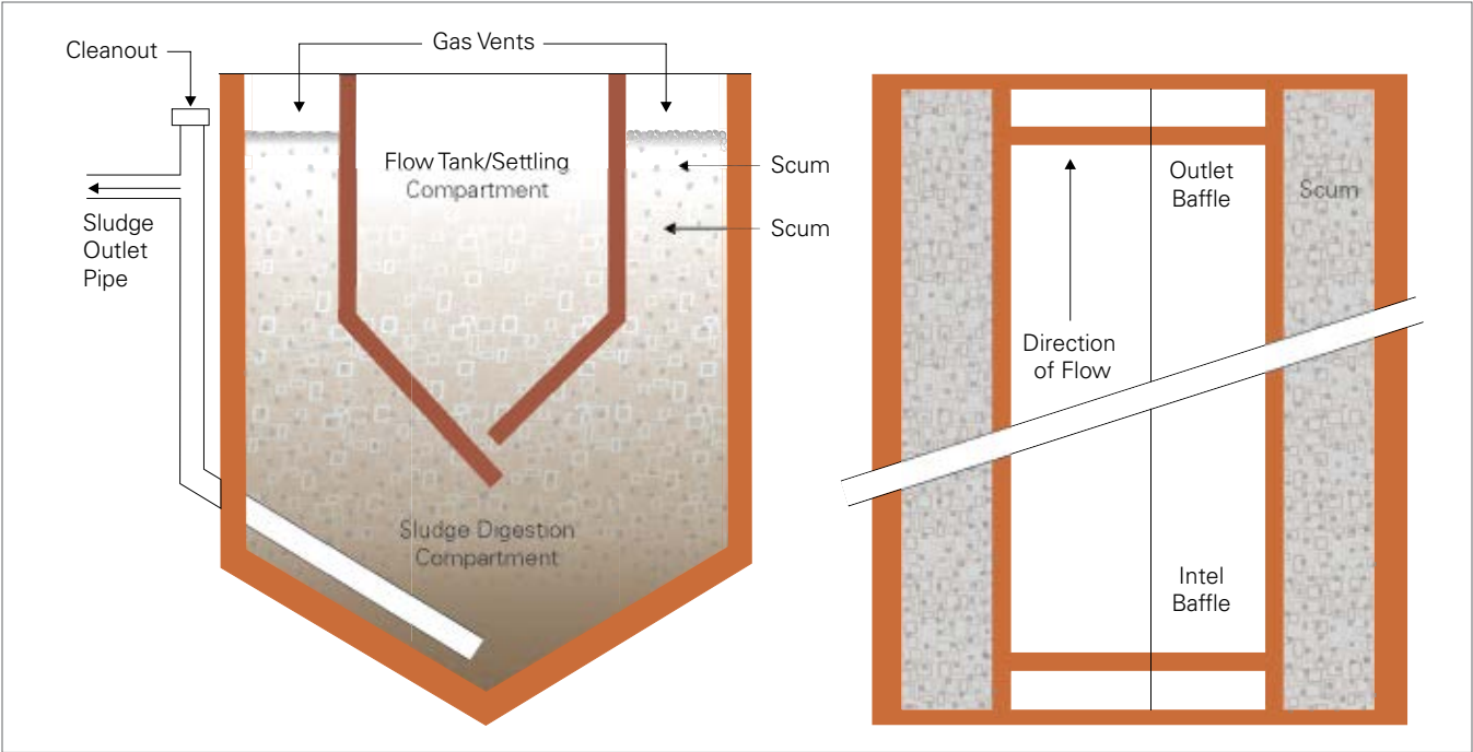
Figure 7.8: An Imhoff tank
