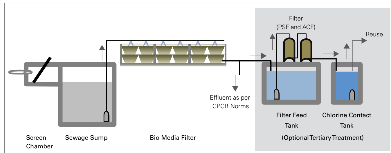
Figure 7.7: Schematic diagram showing process flow of the Tiger Bio Filter
