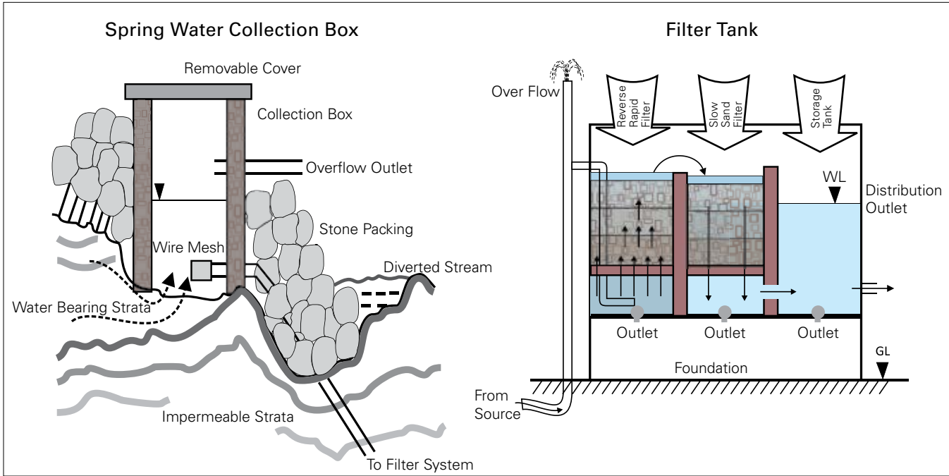
Figure 2.3: Spring based water supply
