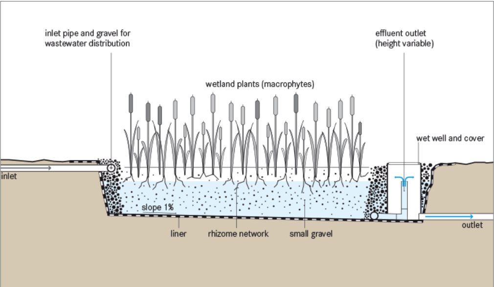
Figure 7.4: Cross-section of subsurface-flow constructed wetland
