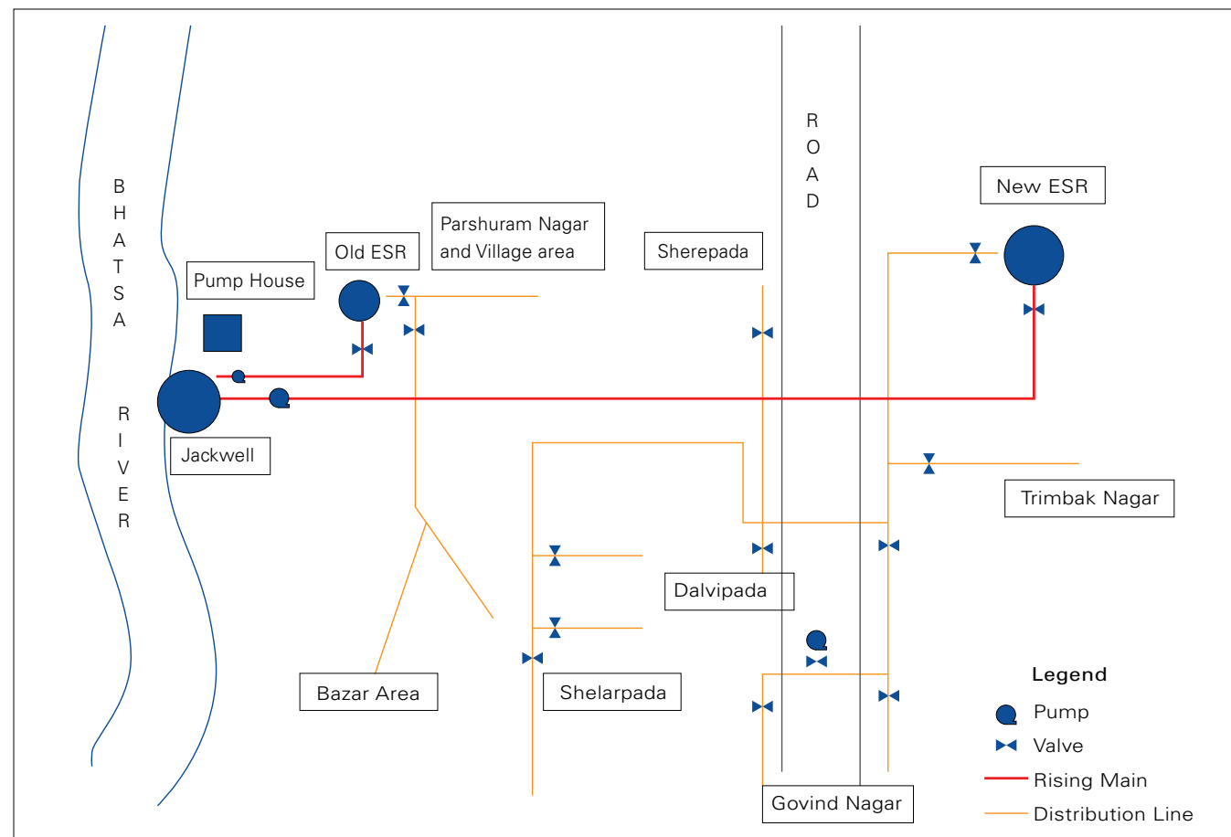
Figure 3B.1: Schematic flow diagram
